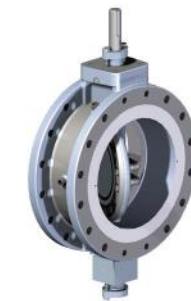
STEAM JACKET BODY/ TRACED DISC AND SHAFT
