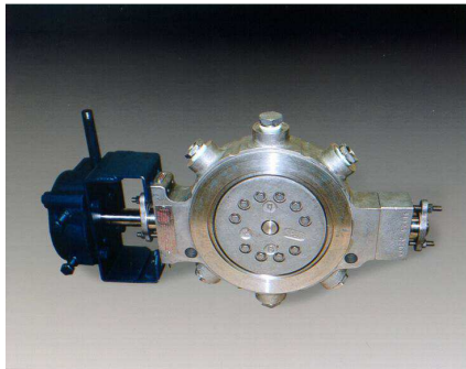
8 CI150 Wafer Nickel 200 with Integral Jacket Caustic Soda Service
