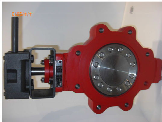
8 CI150 Lug WCB with Impreglon 222M CoatingxCF8M Trim
