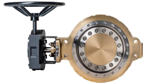
16 CL150 Wafer Replaceable Seat NiAlBzxMonel
