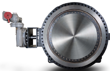
72 CI150 Lug CF8M Downstream View
