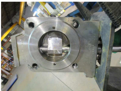
3 CL150 Lug Titanium Gr 2 x Gr 5 Incoming
