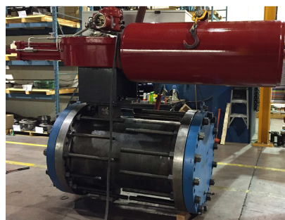
30 CL300 DF Long WCB Pressure Testing
