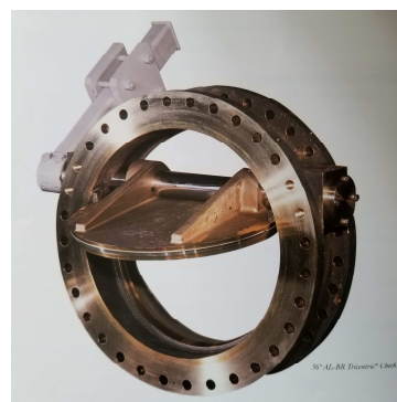
TRICENTRIC Check Valve 36 Cl150 Bronze
