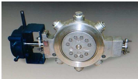
8 CL150 Wafer Nickel 200 Intergral Jacket Caustic Service
