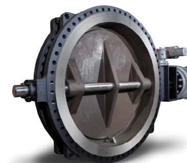
72 CL150 DF Special WCB Jacketed Body and Shaft Tracing
